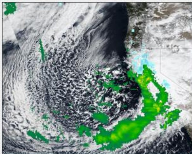
Atmospheric Rivers
